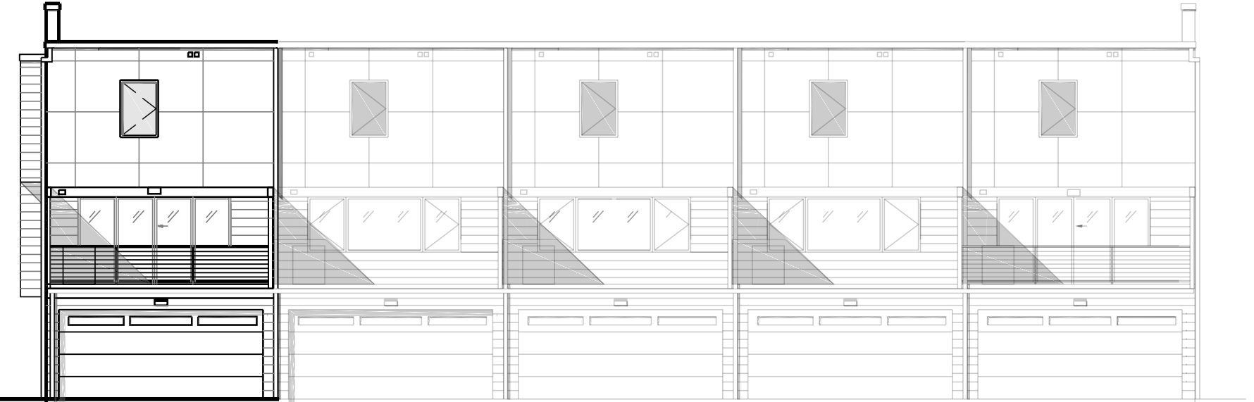
NORTH ELEVATION
