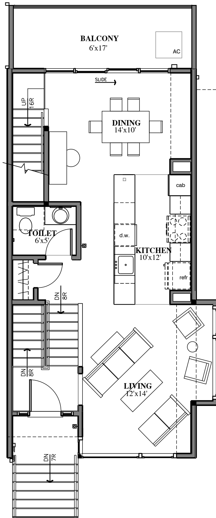
MAIN FLOOR
