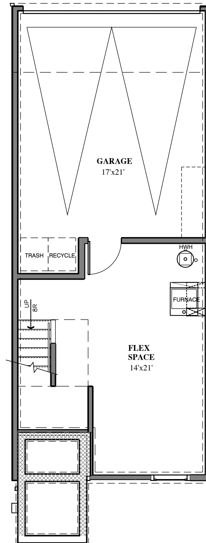
GRADE LEVEL
